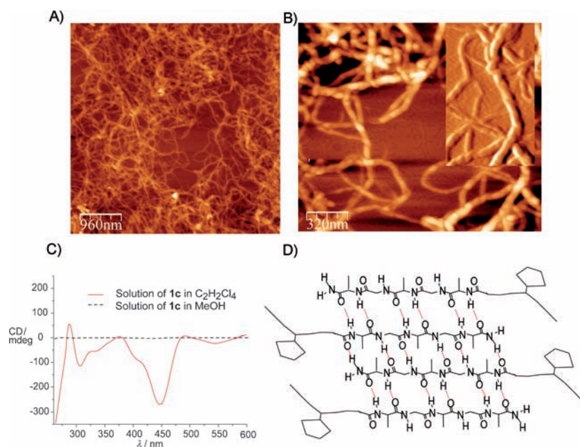
Figure 2. A and B) AFM images of 1c from C 2 H 2 Cl 4 solutions on mica surfaces (5 μm × 5 μm and 1.6 μm × 1.6 μm). C) CD spectra of 1c in MeOH (black spectrum) and in C 2 H 2 Cl 4 (red spectrum). D) Proposed secondary structure (i.e. β-sheet arrangements in antiparallel fashion) of 1c in halogenated solvents.
